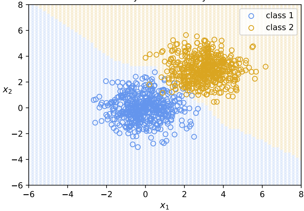
Decision boundary determined by KDEClassifier
